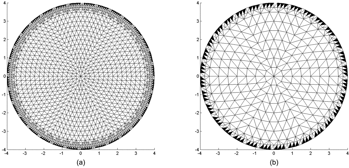
Fig. 1. FEM meshes for (a) forward solver and (b) inverse solver. Locations of the electrodes are marked with darkened elements.
